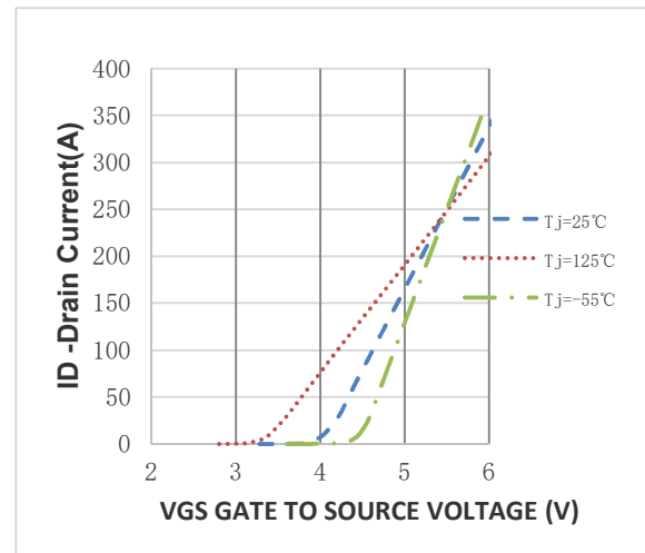
Figure 10. Transfer Characteristics
